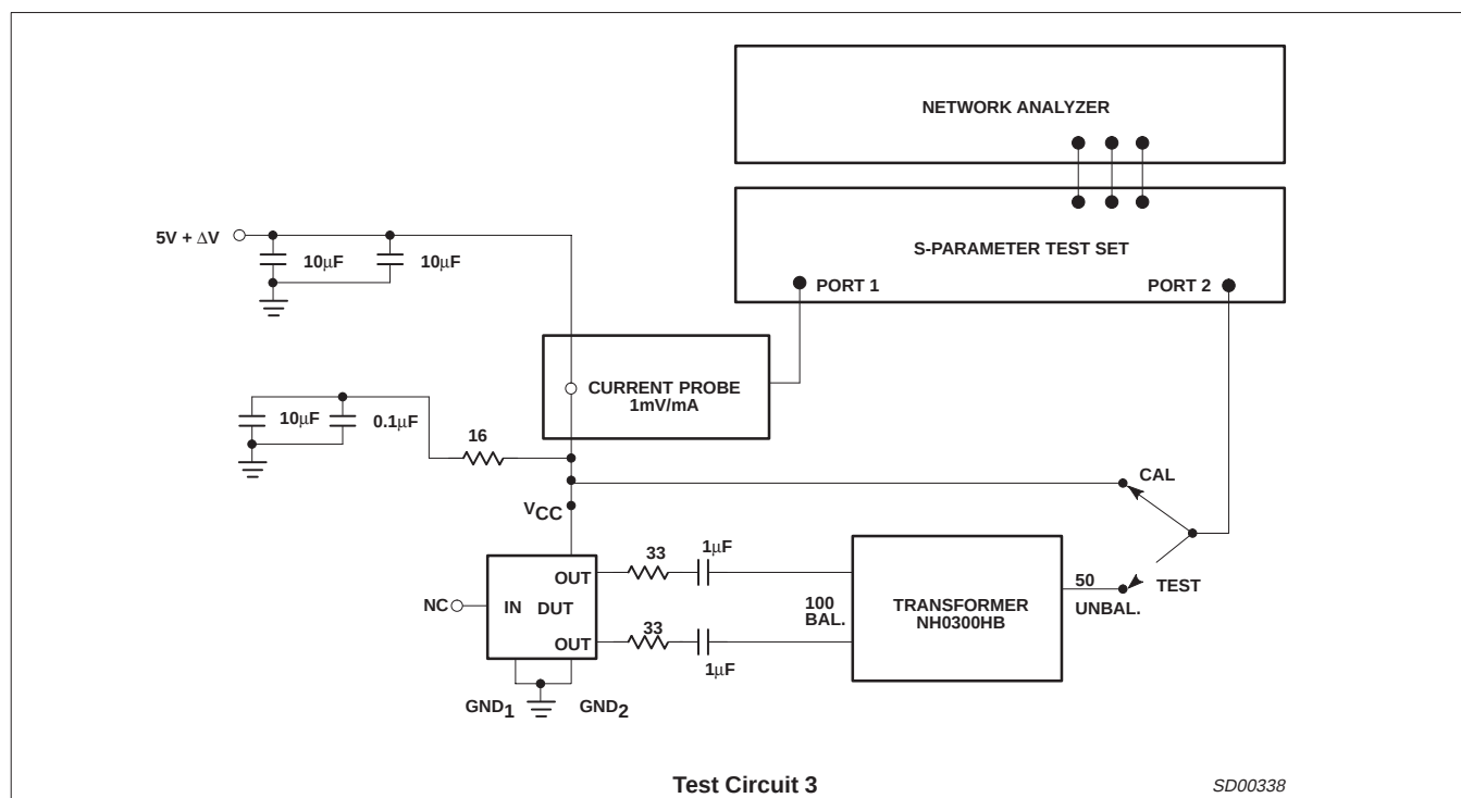
Figure 3. Test Circuit 3
